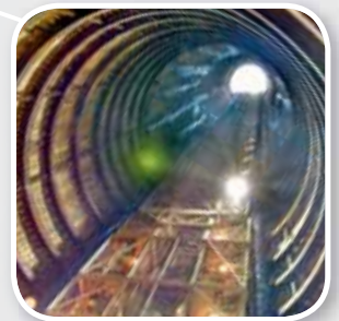
A86 Duplex emergency well, France
